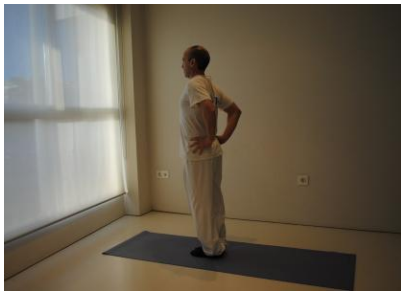
TADASANA
